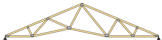
FLAT VAULT
