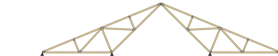
DOUBLE INVERTED
