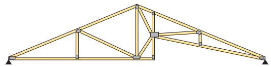
STUDIO VAULT
