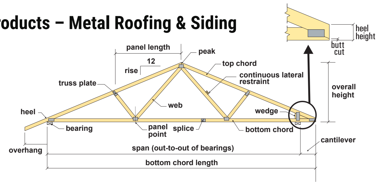
STANDARD ROOF TRUSS CONFIGURATIONS
