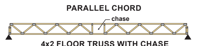
4x2 FLOOR TRUSS WITH CHASE
