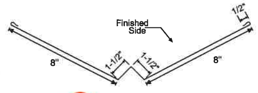
#16 Valley Flashing (Not Shown)
