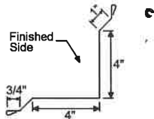
#3 Inside Corner
