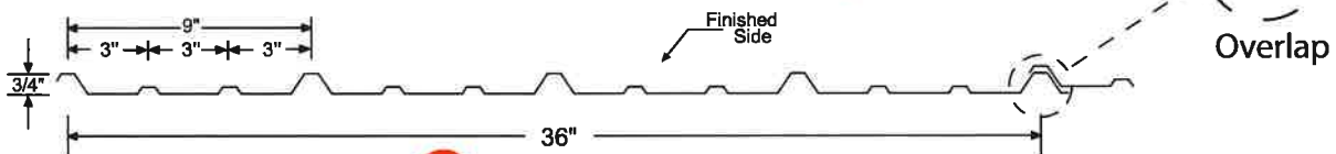
#20 Master Rib Metal Panel
