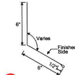
#11 Universal Endwall Flashing
