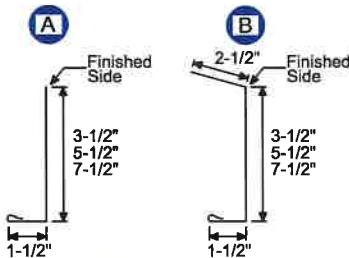
#10 Fascia Trim
