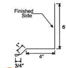
#14 Sidewall Flashing (Not Shown)
